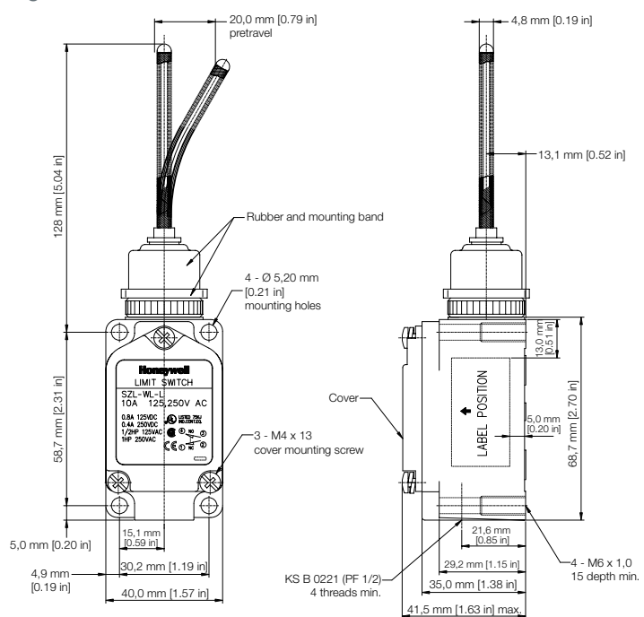
Figure 12. SZL-WL-L
