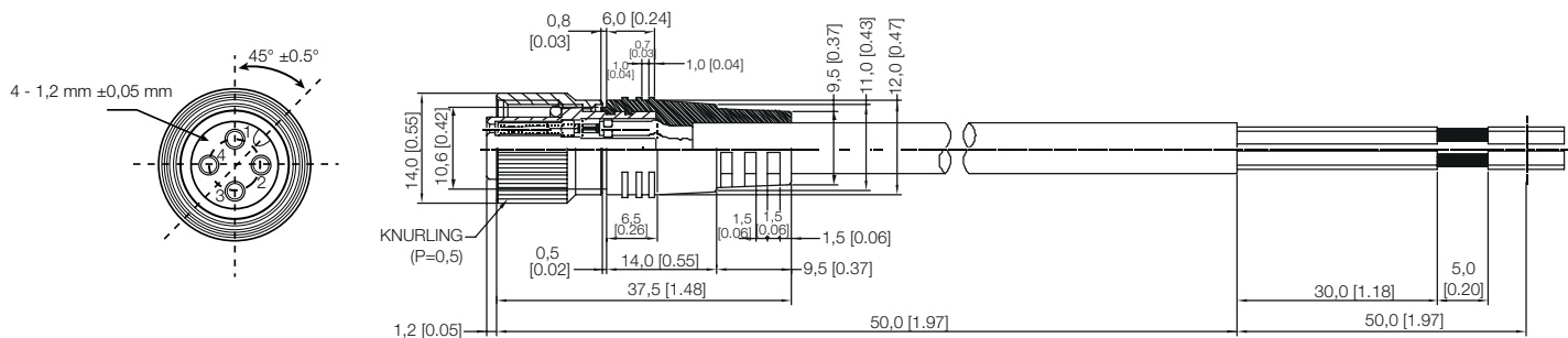
Figure 23. ZLC-4DSF-__
