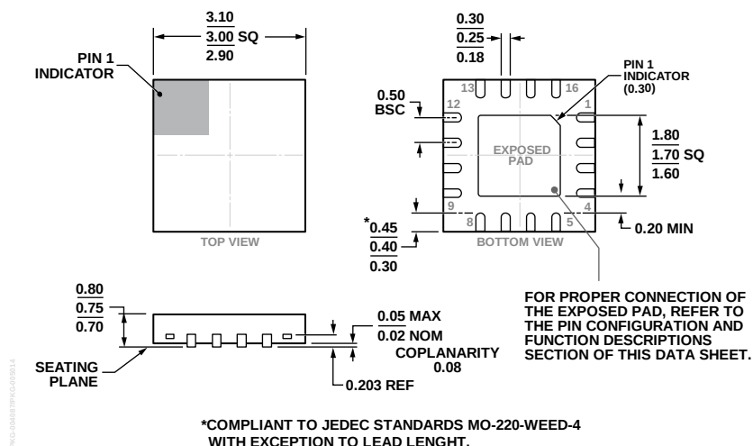
Figure 37. 16-Lead Lead Frame Chip Scale Package [LFCSP_WQ] 3 mm x 3 mm Body, Very Very Thin Quad (CP-16-33) Dimensions shown in millimeters
