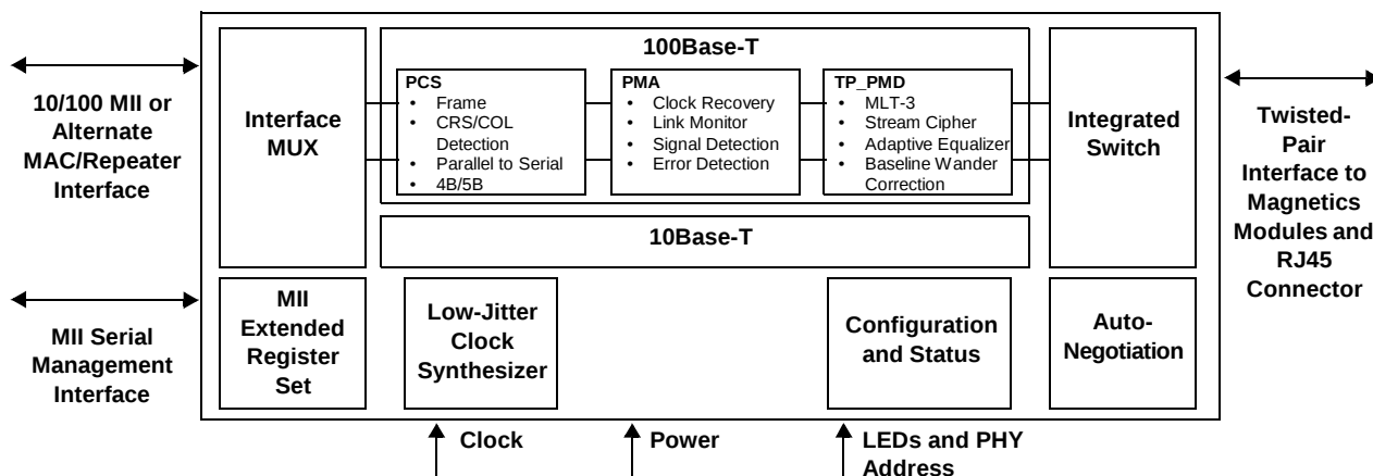
ICS1893 Block Diagram
