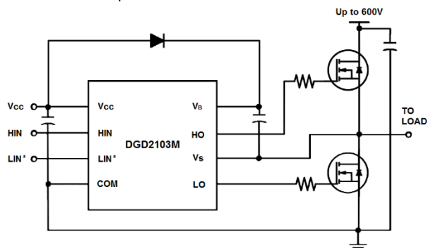
Typical Configuration
