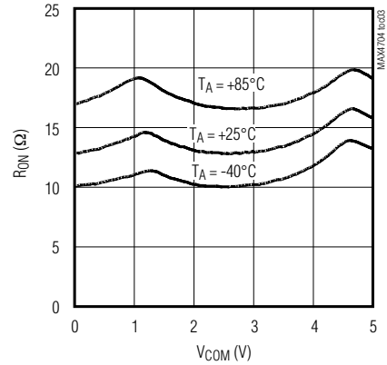
ON-RESISTANCE vs. V_{COM} ( V_+ = 5\text{V} )
