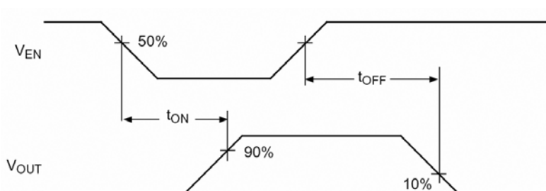
Figure 1b. MIC2544A-2/MIC2548A-2
