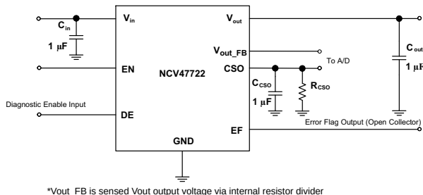
Figure 1. Application Schematic
