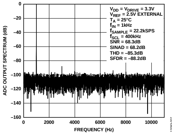
Figure 11. 10 kHz FFT, V_{DD} = 3.0V , V_{REF} = 2.5V External
