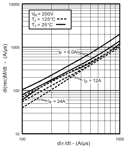
Fig. 17 - Typical dl_{(rec)M}/dt vs di_F/dt
