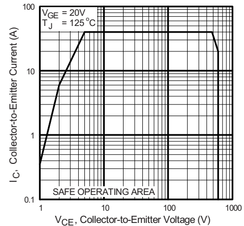
Fig. 12 - Turn-Off SOA
