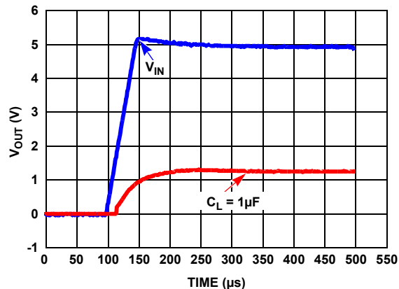
FIGURE 12. TURN ON TIME WITH 1 \mu F
