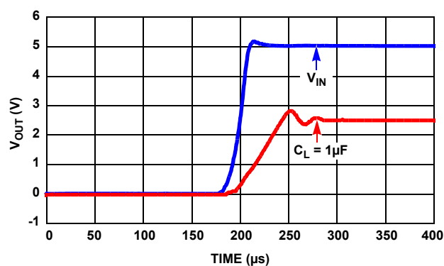
FIGURE 27. TURN-ON TIME WITH 1 \mu\text{F}
