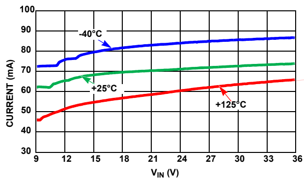
FIGURE 65. SHORT-CIRCUIT TO V_{IN}
