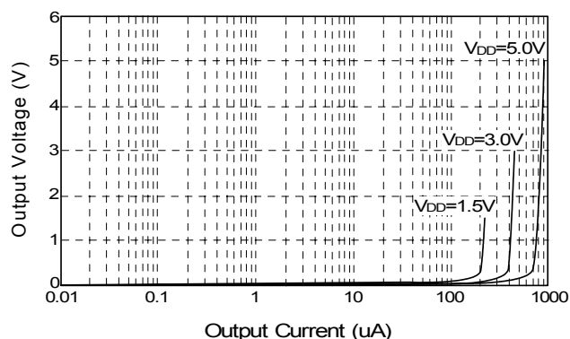
Output Voltage vs. Output Current (SINK)
