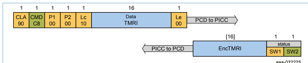
Figure 40. CommitReaderID command protocol
