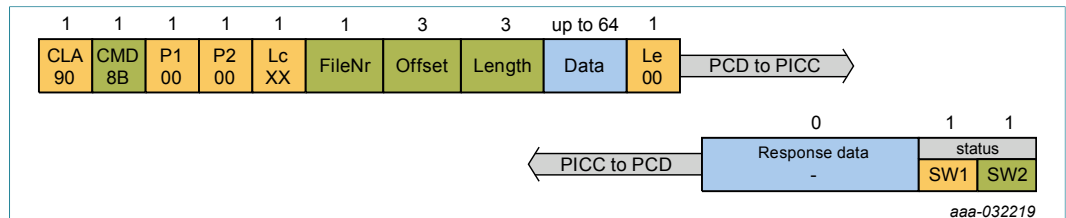
Figure 35. WriteRecord command protocol
