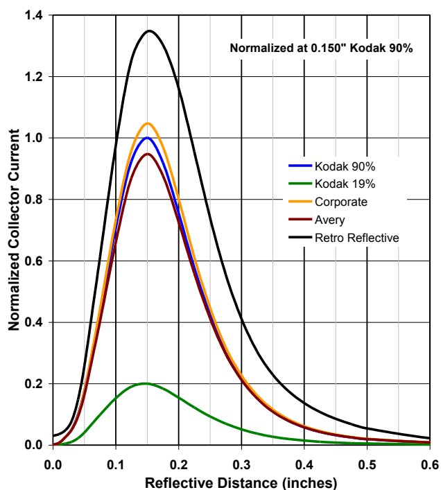
OPB702D - Collector Current vs Distance
