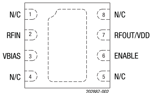
Figure 2. SKY67153-396LF Pinout (Top View)
