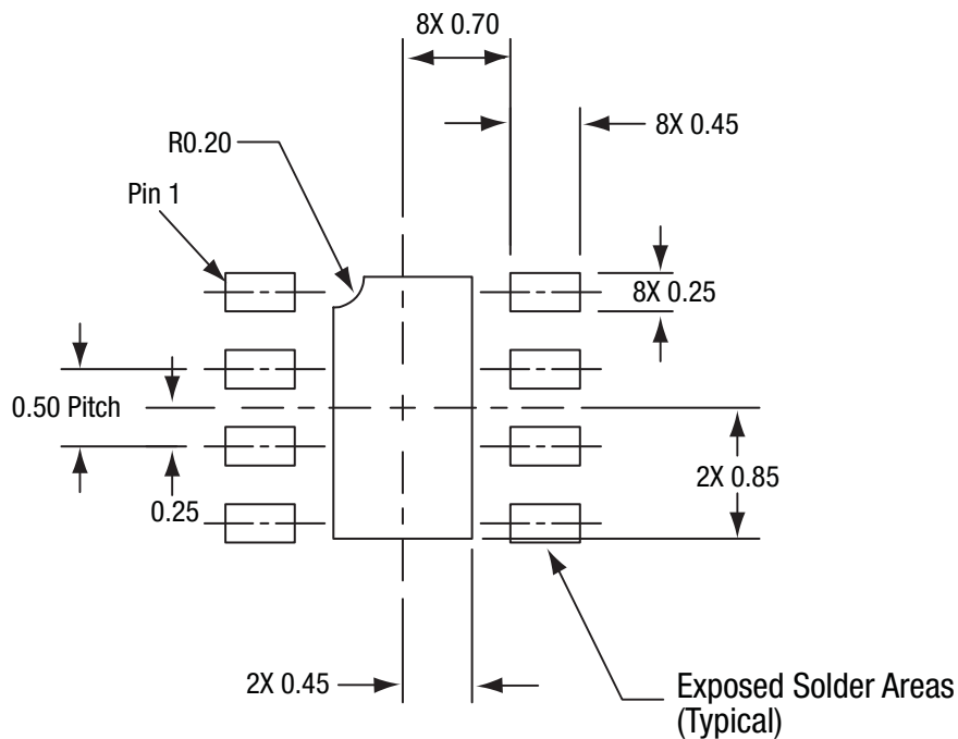
Figure 26. SKY67153-396LF PCB Layout Footprint (Top View)
