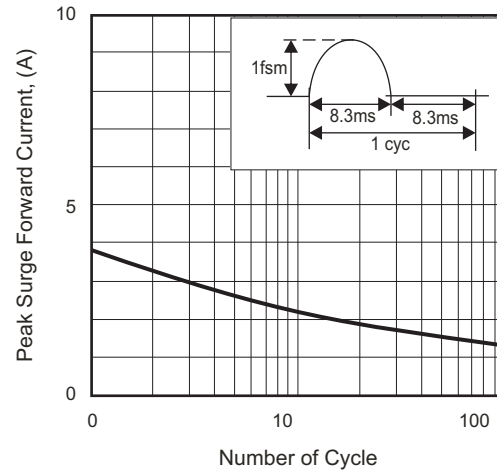
Fig.4 - IFSM-Cycle Characteristics
