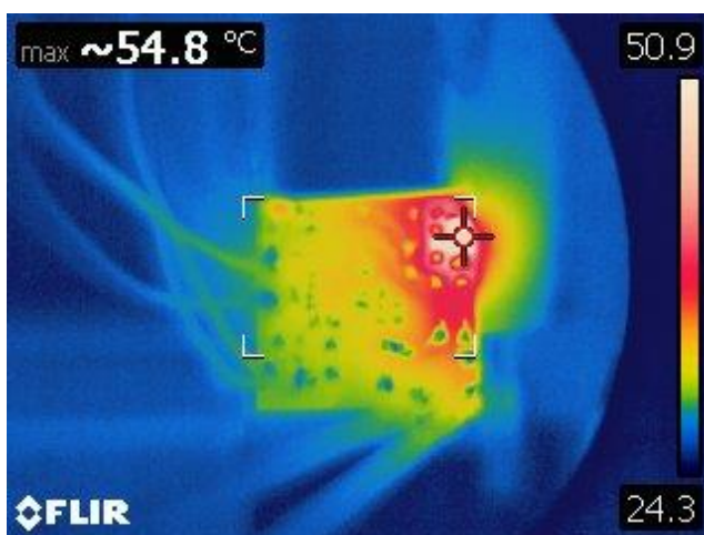
Figure 17 – Measured Temperature at 0.3 W, Ambient Temperature = 24 °C. VR1 – Zener Diode. Spot Temperature = 54.8 °C
