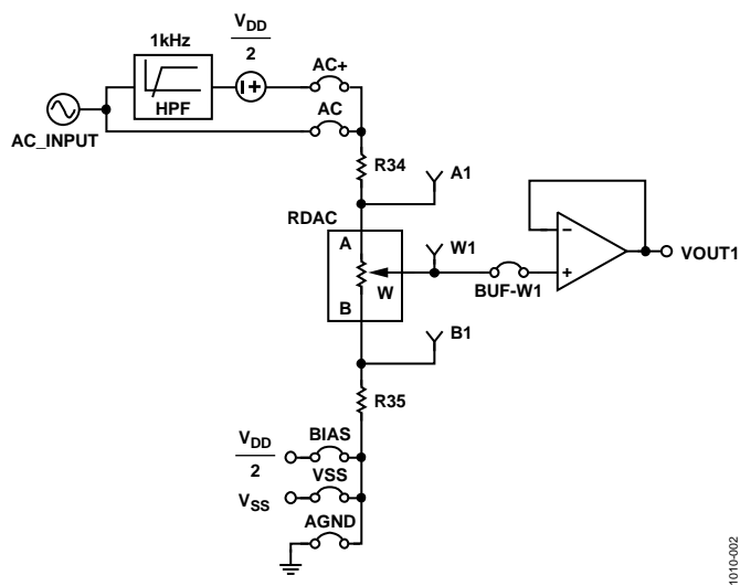
Figure 2. DAC
