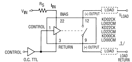
(B) 2 TERMINAL INPUT (OPEN COLLECTOR TTL DRIVE)
