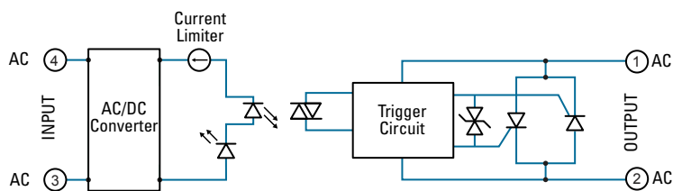
GN Series AC Control
