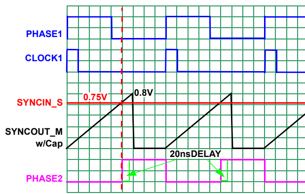
FIGURE 35. SYNCHRONIZATION WAVEFORMS
