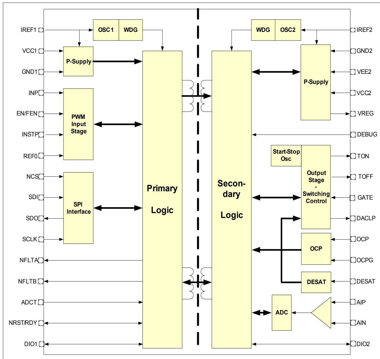
Figure 2-2 Block Diagram
