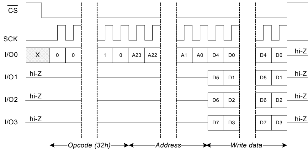
Figure 35. QIW Instruction
