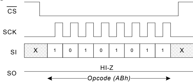
Figure 59. EXSLP Instruction in SPI Mode
