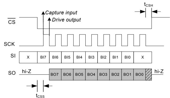
Figure 4. SPI Mode 0
