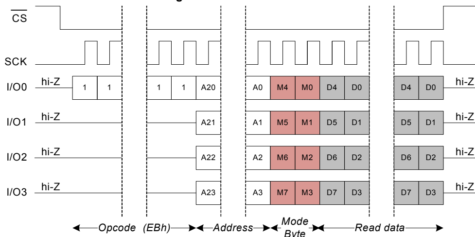
Figure 29. QIOR Instruction
