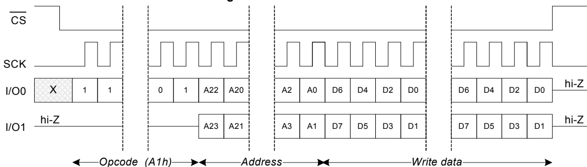
Figure 36. DIOW Instruction
