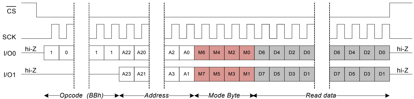
Figure 28. DIOR Instruction
