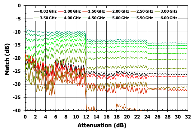
Output Return Loss vs Attenuation
