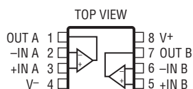
MS8 PACKAGE 8-LEAD PLASTIC MSOP T_{JMAX} = 150^\circ\text{C} , \theta_{JA} = 250^\circ\text{C/W}
