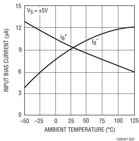
Input Bias Currents vs Temperature
