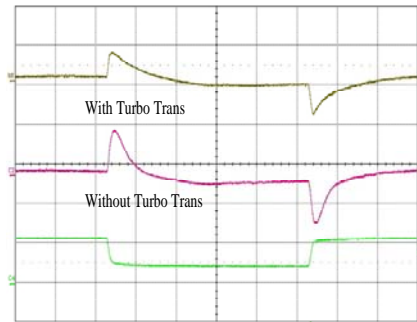
Output voltage response to load current step-change (7.5-22.5-7.5 A) at: T_{ref} = +25^\circ\text{C} , V_i = 5\text{ V} . Top trace: output voltage (100 mV/div.). Middle trace: output voltage (100mV/div.). Bottom trace: load current (20 A/div.). Time scale: (0.1 ms/div.).
