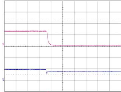
Shut-down enabled by disconnecting V_i at: T_{ref} = +25^\circ\text{C} , V_i = 5\text{ V} , I_o = 30\text{ A} resistive load. Top trace: output voltage (1 V/div.). Bottom trace: input voltage (5 V/div.). Time scale: (0.5 ms/div.).
