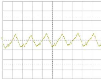
Output voltage ripple at: T_{ref} = +25^{\circ}\text{C} , V_i = 5\text{ V} , I_o = 30\text{ A} resistive load. Trace: output voltage (2 mV/div.). Time scale: (2 \mu\text{s} /div.).
