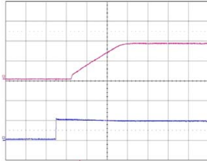
Start-up enabled by connecting V_i at: T_{ref} = +25^{\circ}\text{C} , V_i = 5\text{ V} , I_o = 30\text{ A} resistive load. Top trace: output voltage (1 V/div.). Bottom trace: input voltage (5 V/div.). Time scale: (5 ms/div.).
