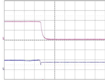
Shut-down enabled by disconnecting V_i at: T_{ref} = +25^{\circ}\text{C} , V_i = 5\text{ V} , I_o = 30\text{ A} resistive load. Top trace: output voltage (1 V/div.). Bottom trace: input voltage (5 V/div.). Time scale: (0.5 ms/div.).
