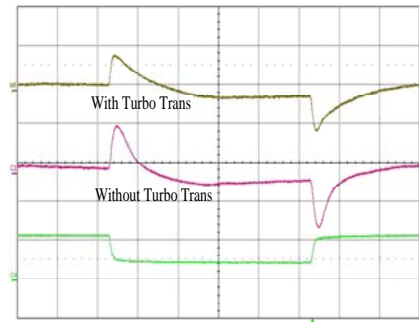
Output voltage response to load current step-change (7.5-22.5-7.5 A) at: T_{ref} = +25^{\circ}\text{C} , V_i = 5\text{ V} . Top trace: output voltage (100 mV/div.). Middle trace: output voltage (100mV/div.). Bottom trace: load current (20 A/div.). Time scale: (0.1 ms/div.).
