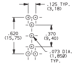
PC MOUNTING
