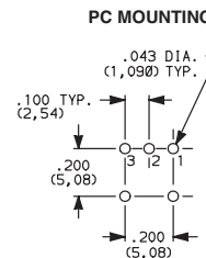
T101J6ABE2 Horizontal Actuation SPDT
