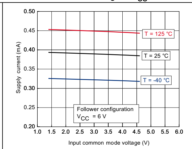
Figure 7. Supply current (per channel) vs. input common mode voltage at V_{CC} = 6 V
