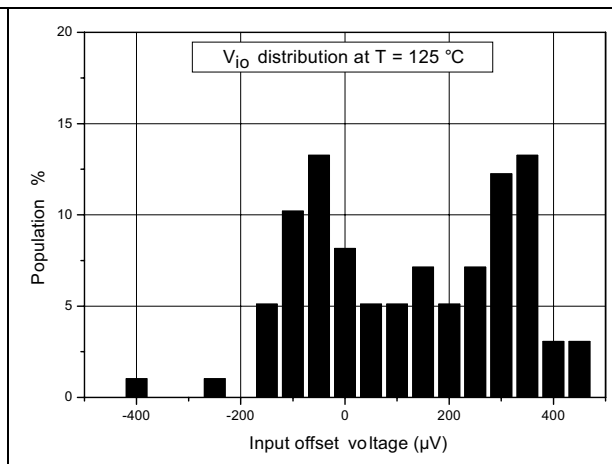
Figure 3. V_{io} distribution at V_{CC} = \pm 15 V and T = 125 °C
