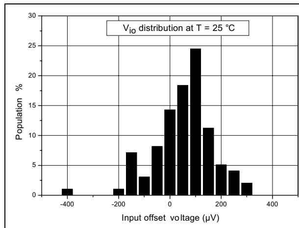
Figure 2. V_{io} distribution at V_{CC} = \pm 15 V and T = 25 °C
