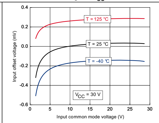
Figure 5. Input offset voltage vs. input common mode voltage at V_{CC} = 30 V
