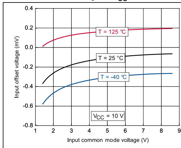
Figure 4. Input offset voltage vs. input common mode voltage at V_{CC} = 10 V
