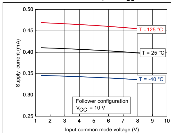
Figure 8. Supply current (per channel) vs. input common mode voltage at V_{CC} = 10\text{ V}
