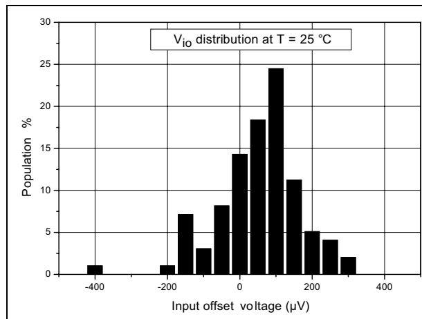
Figure 2. V_{io} distribution at V_{CC} = \pm 15 V and T = 25 °C
