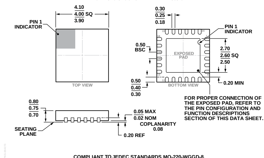
Figure 39. 24-Lead Lead-frame Chip Scale Package [LFCSP_WQ] 4 mm × 4 mm Body, Very Very Thin Quad (CP-24-15)
