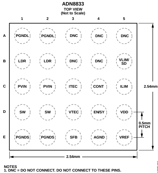
Figure 2. WLCSP Pin Configuration (Top View)
