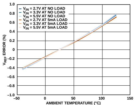
Figure 10. V_{REF} Error vs. Ambient Temperature
