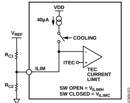
Figure 29. Using a Resistor Divider to Set the TEC Current Limit
