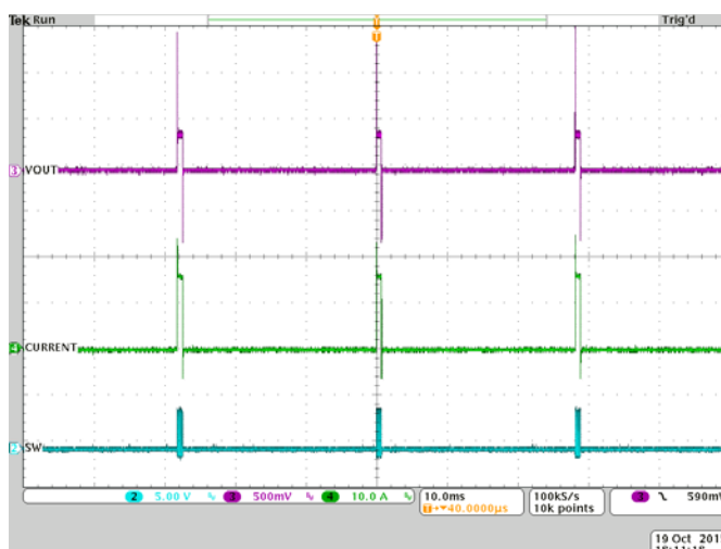
Figure 20: Hiccup mode during short-circuit protection
