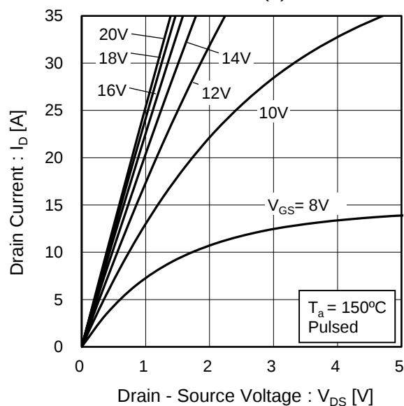
Fig.7 T_j = 150^\circ\text{C} Typical Output Characteristics(II)
