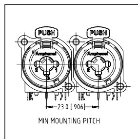
C TYPE LOW PROFILE MOUNTING PITCH
