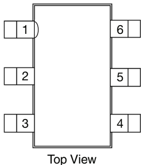
Figure 3 - TSOT23-6 Package
