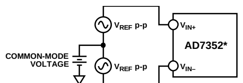
Figure 19. Differential Input Definition
