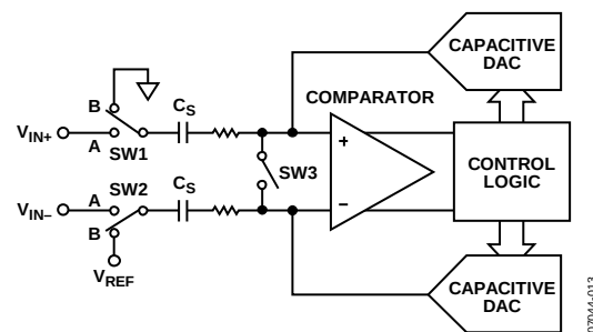
Figure 15. ADC Conversion Phase
