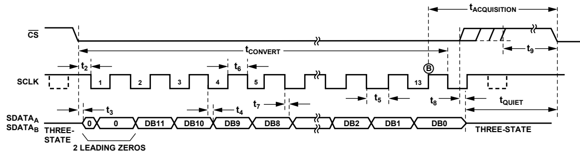
Figure 30. Serial Interface Timing Diagram
