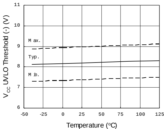
Figure 18. V_{\text{CC}} Undervoltage Threshold (-) vs. Temperature
