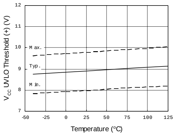
Figure 17. V_{\text{CC}} Undervoltage Threshold (+) vs. Temperature
