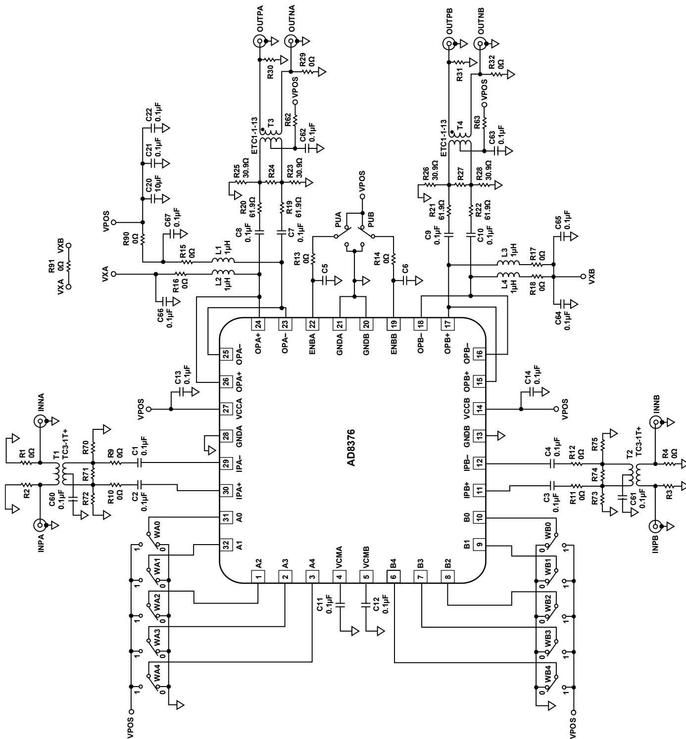
Figure 47. AD8376 Evaluation Board Schematic
