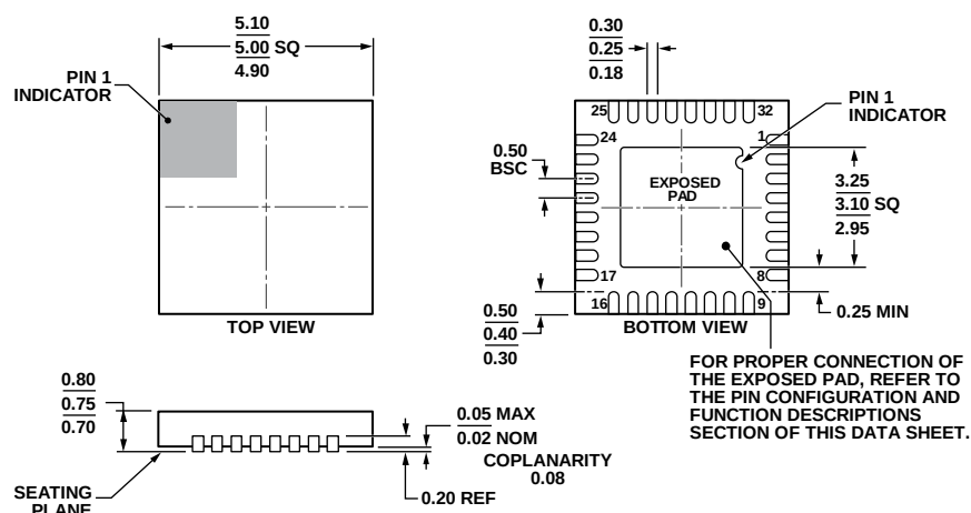
Figure 52. 32-Lead Lead Frame Chip Scale Package [LFCSP_WQ] 5 mm × 5 mm Body, Very Very Thin Quad (CP-32-7)
