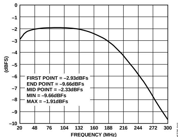
Figure 41. Measured Frequency Response of Wideband ADC Interface Depicted in Figure 39
