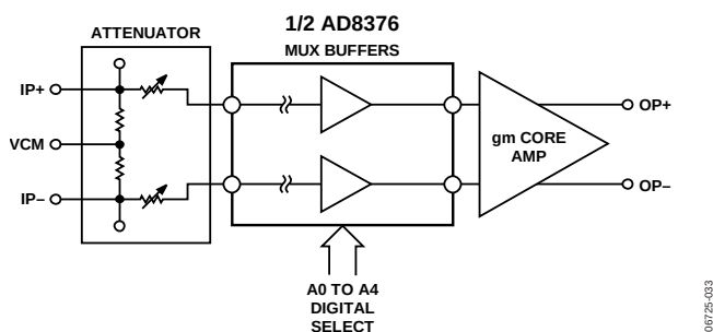
Figure 33. Simplified Schematic
