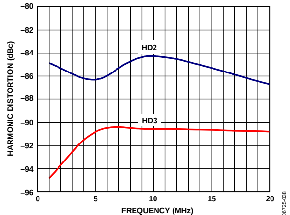
Figure 38. Harmonic Distortion vs. Frequency Using Resistive Pull-Ups
