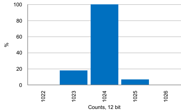
Figure 11-45. SAR ADC Noise Histogram, 1 msp, Internal Reference Bypassed
