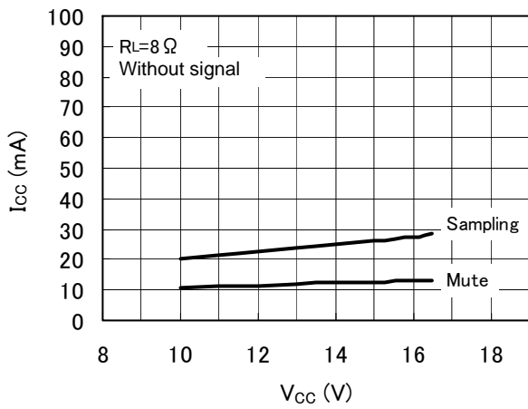
Fig. 11 Current consumption - Power supply voltage
