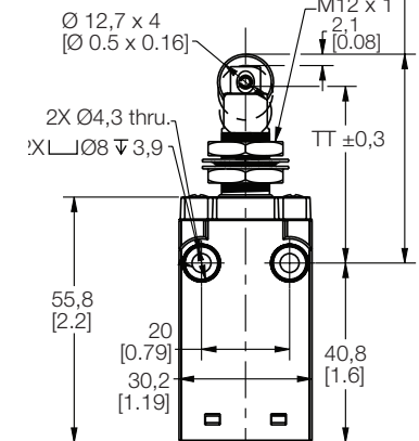
Figure 13. Panel-Mount Roller Plunger P Dimensions
