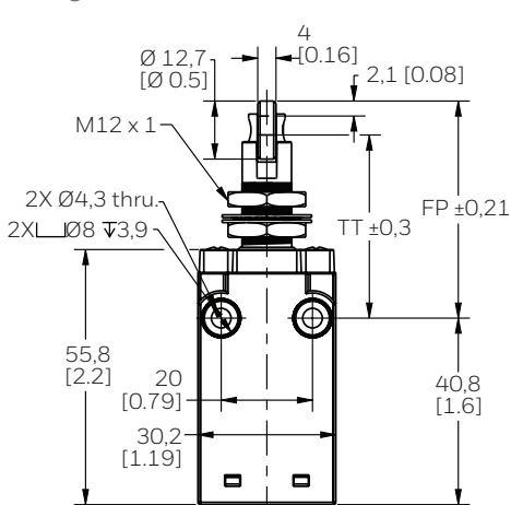
Figure 14. Panel-Mount Cross Roller Plunger Q Dimensions
