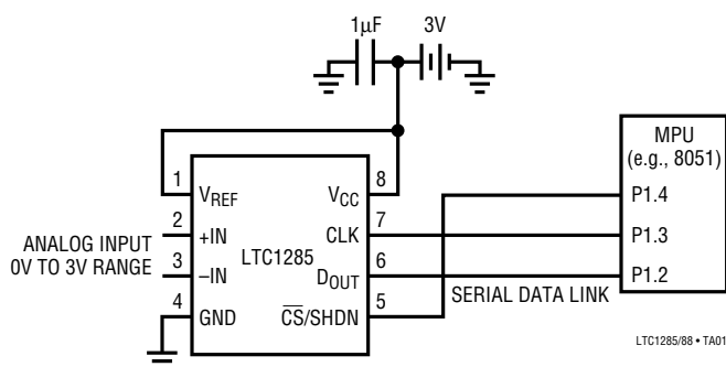
12μW, S0-8 Package, 12-Bit ADC Samples at 200Hz and Runs Off a 3V Supply
