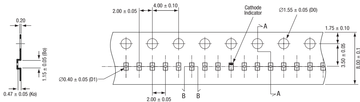
Figure 10. SOD-882 Package Dimension Drawing
