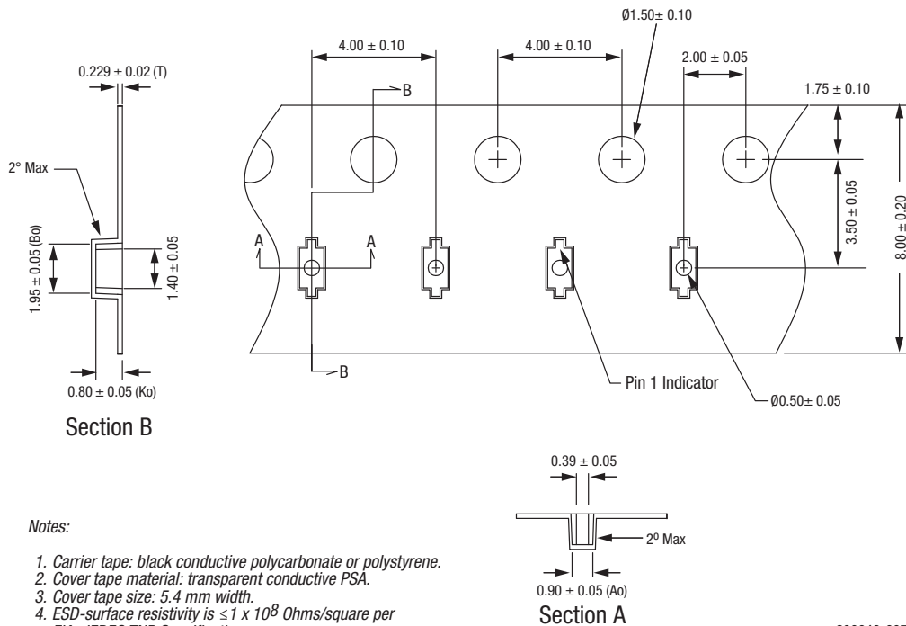
Figure 7. SC-79 Tape and Reel Dimensions
