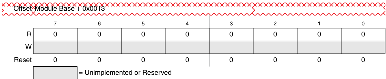
Figure 17-23. Flash Reserved7 Register (FRSV7)
