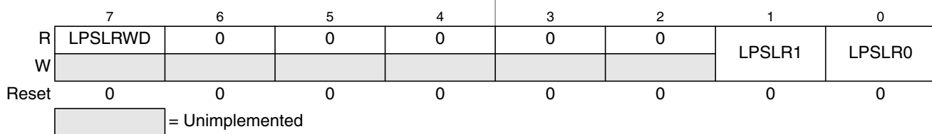
Figure 15-5. LIN Slew Rate Register (LPSLR)
