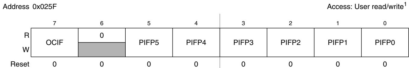
Figure 2-30. Port P Interrupt Flag Register (PIFP)
